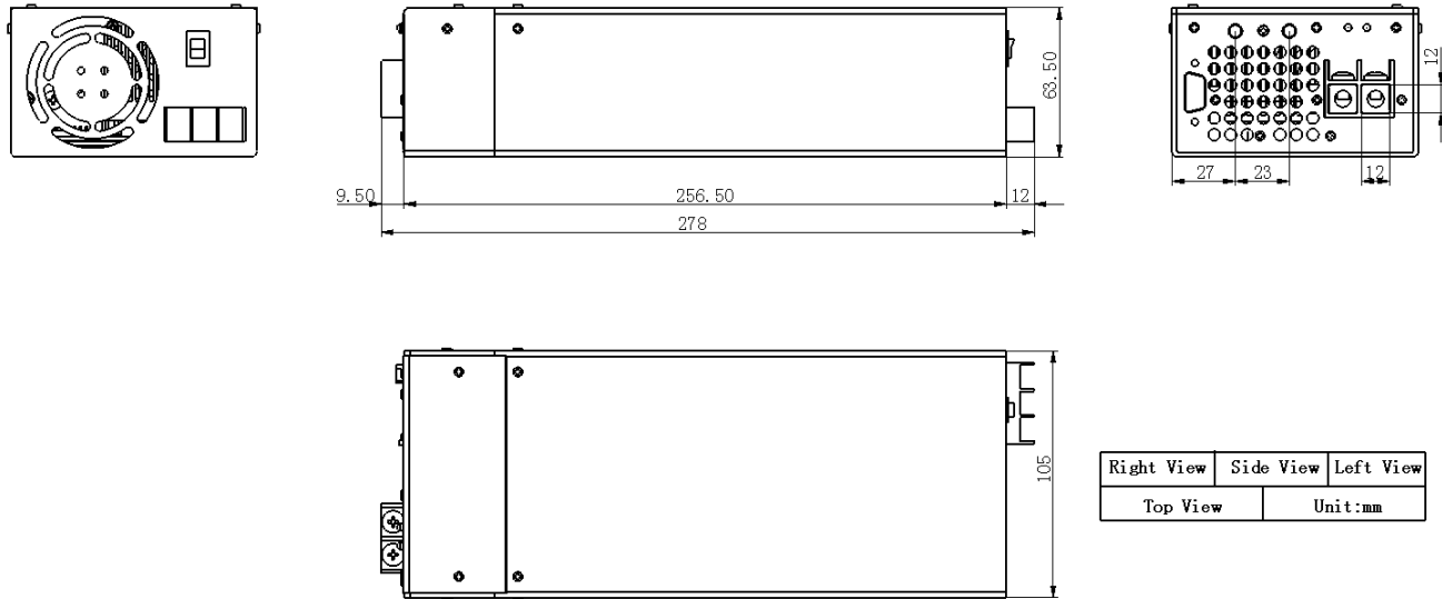
Figure 19. Mechanical Dimensions
